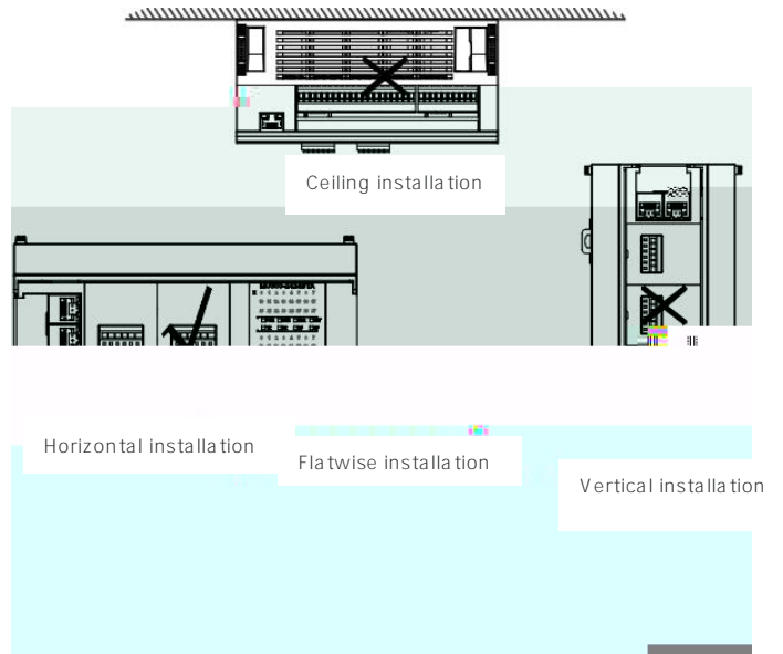
Fig 3-1 Installation position diagram
